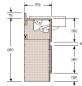
K1 Profile - Semi recessed washbasin profile with upstand
