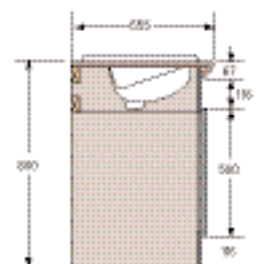
K8 Profile - Fully inset washbasin profile without upstand
