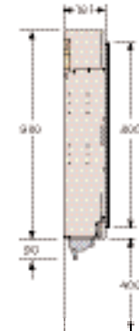
Mirror Dispensing Cabinet 0302040 with B1 Bulk Head wall unit. Note 21mm space for tiling
