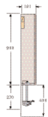
Retractable Towel Dispenser 0302042 with B1 Bulk Head wall unit. Note 270mm clear access space required beneath towel dispenser, 400mm recommended height for bulk head above vanity. Note 10mm space for tiling
