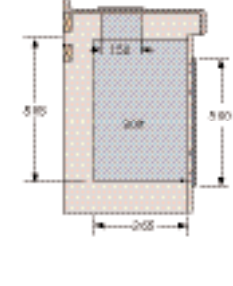
0302044 with K3 profile. Note space available between wall and back of bin for plumbing is a minimum of 70mm dependent on which vanity profile the bin is housed within Bin volume = 30lt Bin width = 300mm
