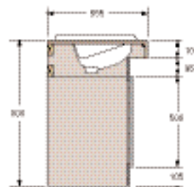
K4 Profile - Fully inset washbasin profile without upstand
