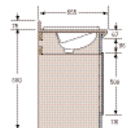
K7 Profile - Fully inset washbasin profile with upstand
