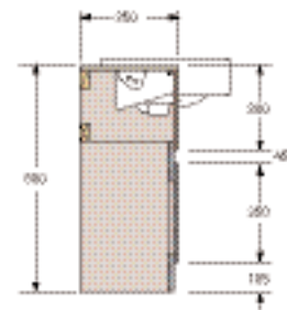
K2 Profile - Semi recessed washbasin profile without upstand
