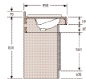
K3 Profile - Fully inset washbasin profile with upstand
