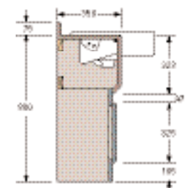
K5 Profile - Semi recessed washbasin profile with upstand
