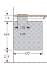
0302043 with K8 vanity top without underframes. Bin volume = 40lt Bin width = 300mm
