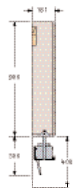
Retractable Soap Dispenser 0302041 with B1 Bulk Head wall unit. Note 300mm clear access space required beneath soap dispenser, 400mm recommended height for bulk head above vanity. Note 10mm space for tiling
