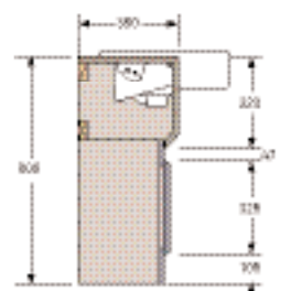
K6 Profile - Semi recessed washbasin profile without upstand
