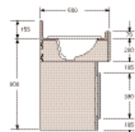
Baby change Profile
