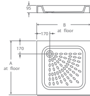
2 Upstand tray
