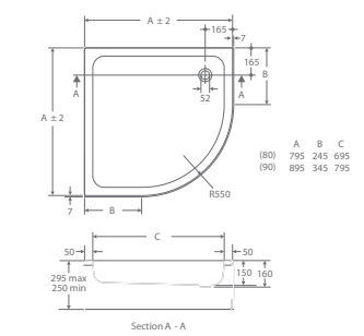
Kielder Quadrant 900
