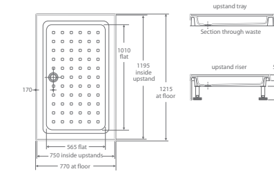
Upstand tray
